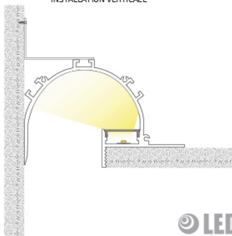
INSTALLATION VERTICALE
